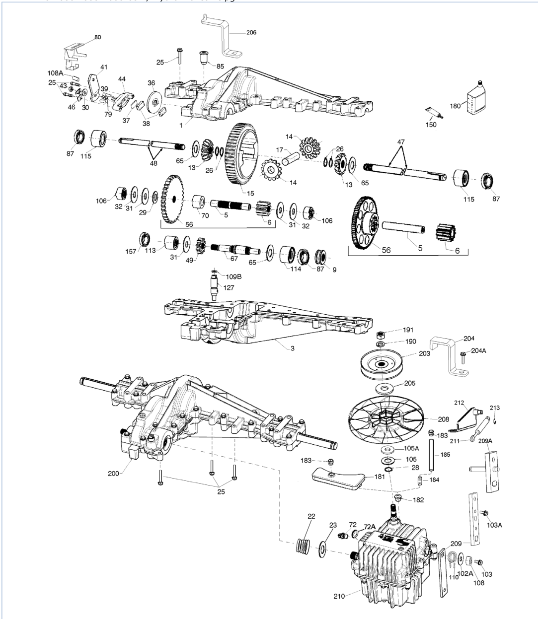
lth2000 2000-2000-031 / Hydro Transaxle pg 1
